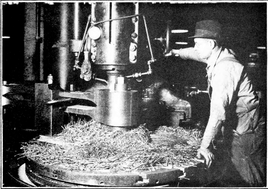
FIGURE 1.- MACHINIST MILLING DOWN PART OF A DRIVE SHAFT FOR A LOCOMOTIVE
