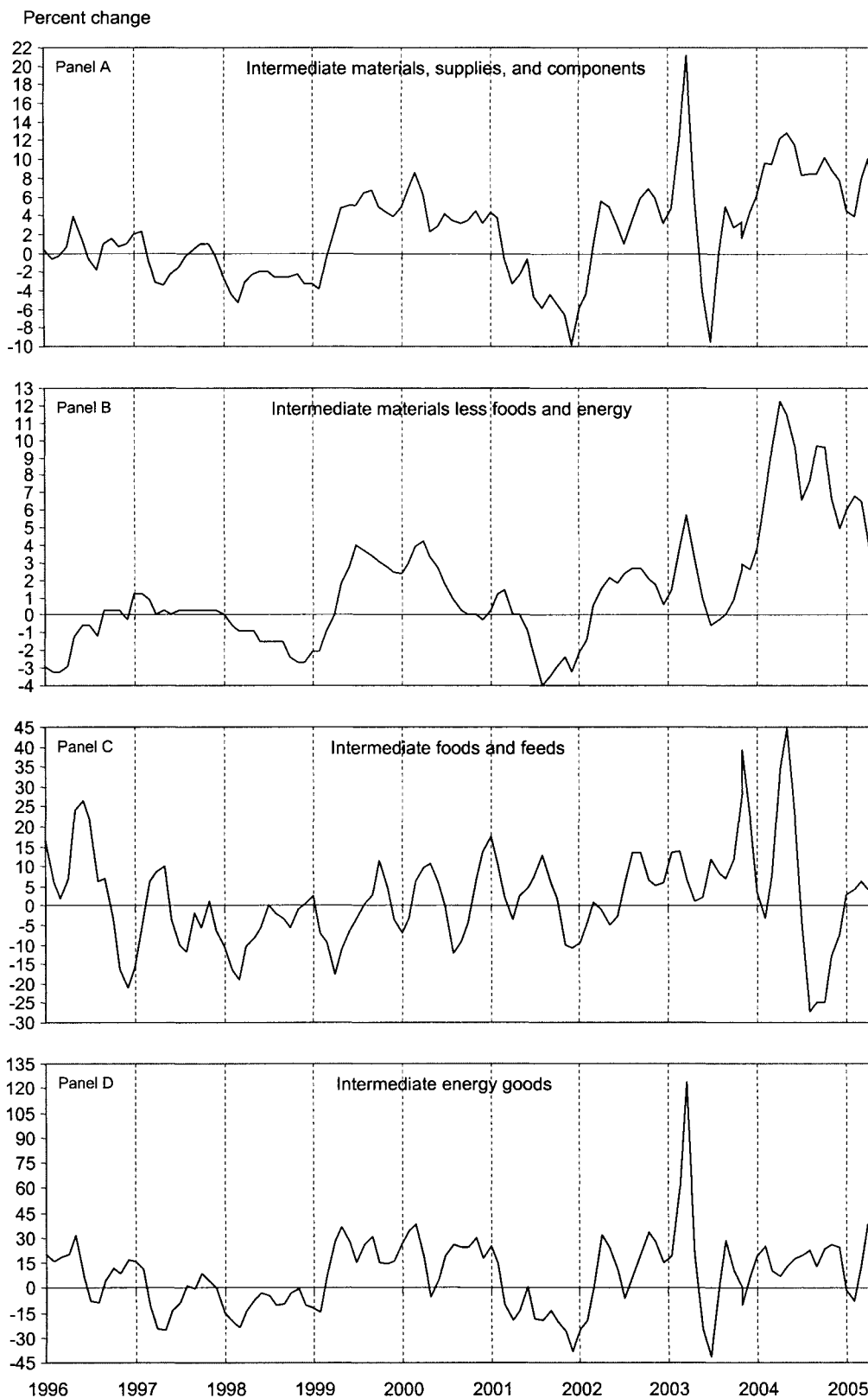
Chart 2. The Intermediate Goods Index and its component indexes, January 1996 through May 2005, 3-month seasonally adjusted annual rates of change
