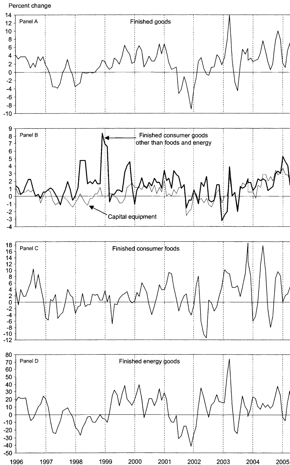
Chart 1. The Finished Goods Index and its component indexes, January 1996 through May 2005, 3-month seasonally adjusted annual rates of change
