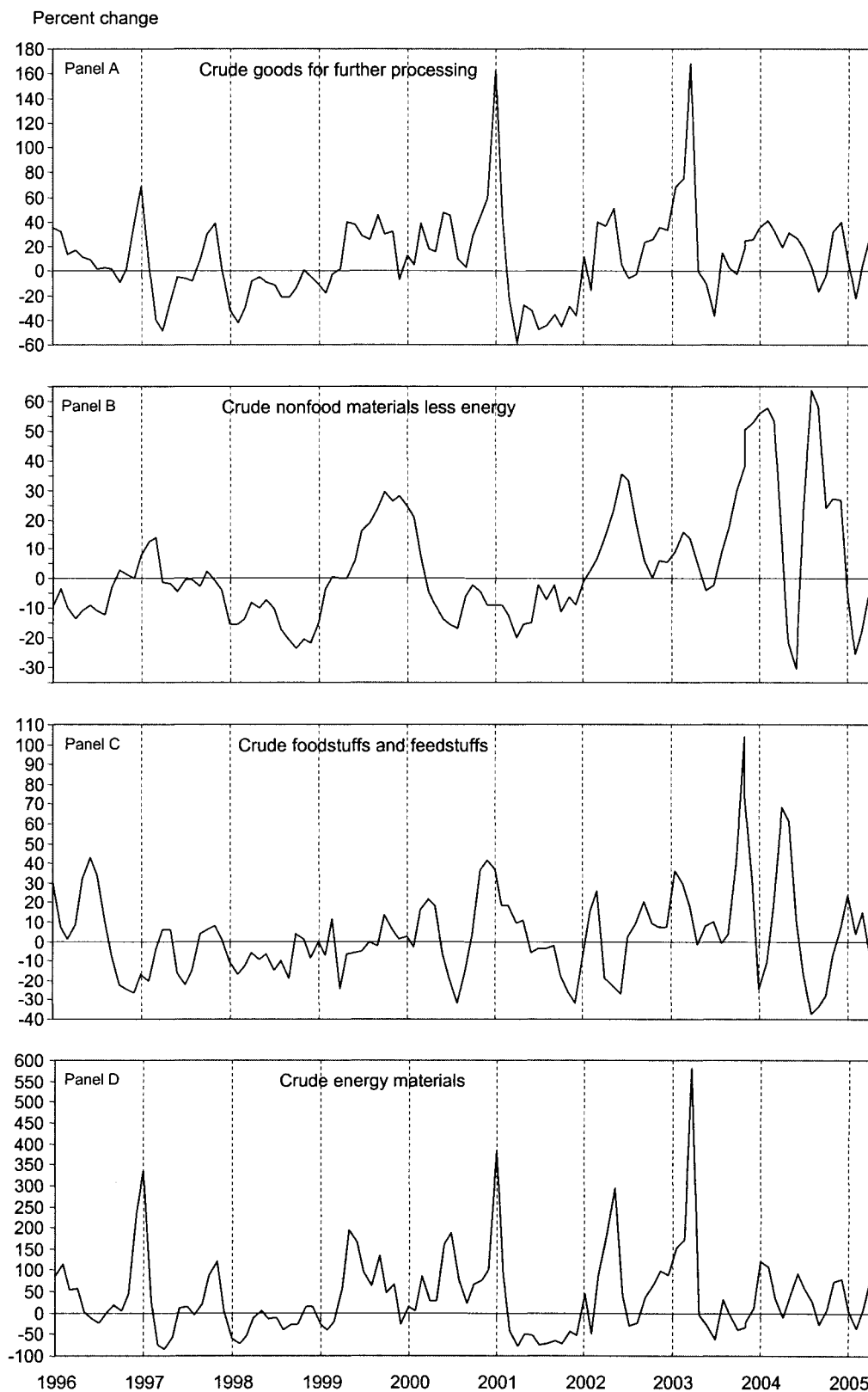
Chart 3. The Crude Goods Index and its component indexes, January 1996 through May 2005, 3-month seasonally adjusted annual rates of change
