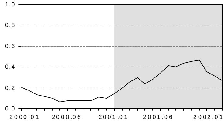
a) Model 1 - Constant Variance and i.i.d. Errors
