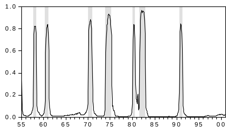
c) Model 3 - Constant Variance and AR(1) Process
