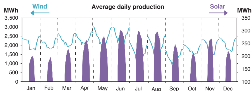
CHART 1 Complementary Wind, Solar Energy Help Stabilize Production
