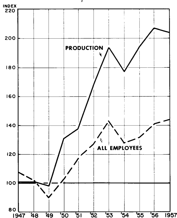
Chart 1. Indexes of Average Monthly Production and Employment in the Electrical Machinery Industry Group, 1947-57 1947-49=100
