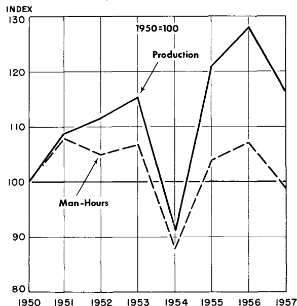
Chart 1. Indexes of Average Monthly Production of Ingots and Steel for Castings and Aggregate Weekly Man-Hours of Production Workers in Blast Furnaces, Steel Works, and Rolling Mills, 1950-57
