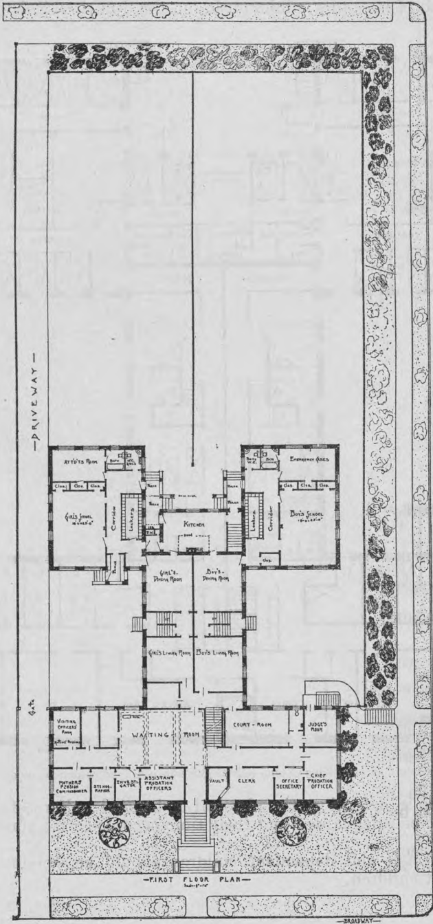
First-floor plan, King County [Seattle] juvenile court and detention home.
