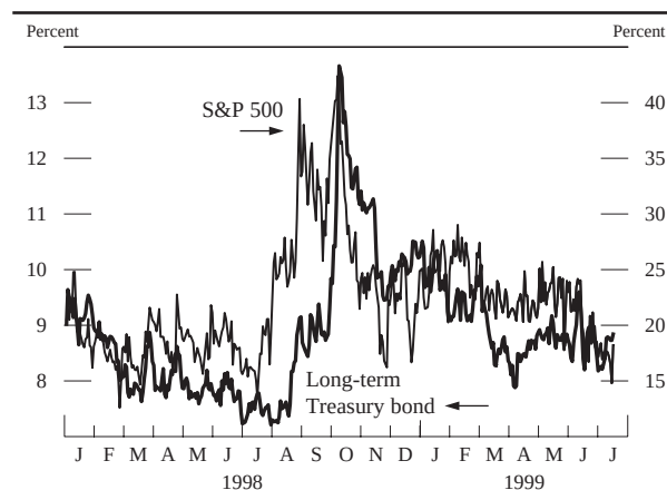
Implied volatilities
