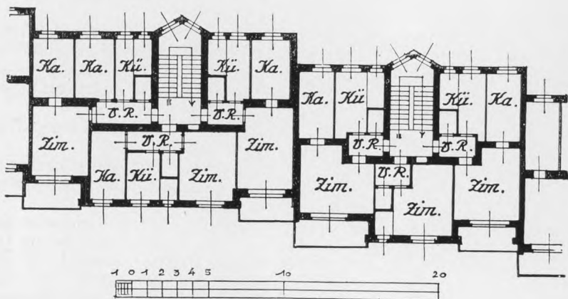
FIGURE 3.—FLOOR PLAN OF APARTMENT ERECTED UNDER VIENNA HOUSING PLAN
