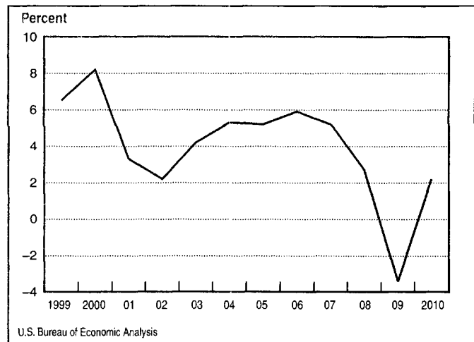
U.S. Compensation, 1999–2010
