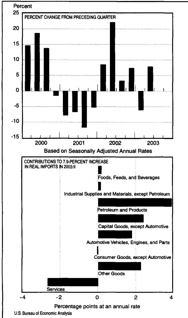
Chart 8. Real Imports
