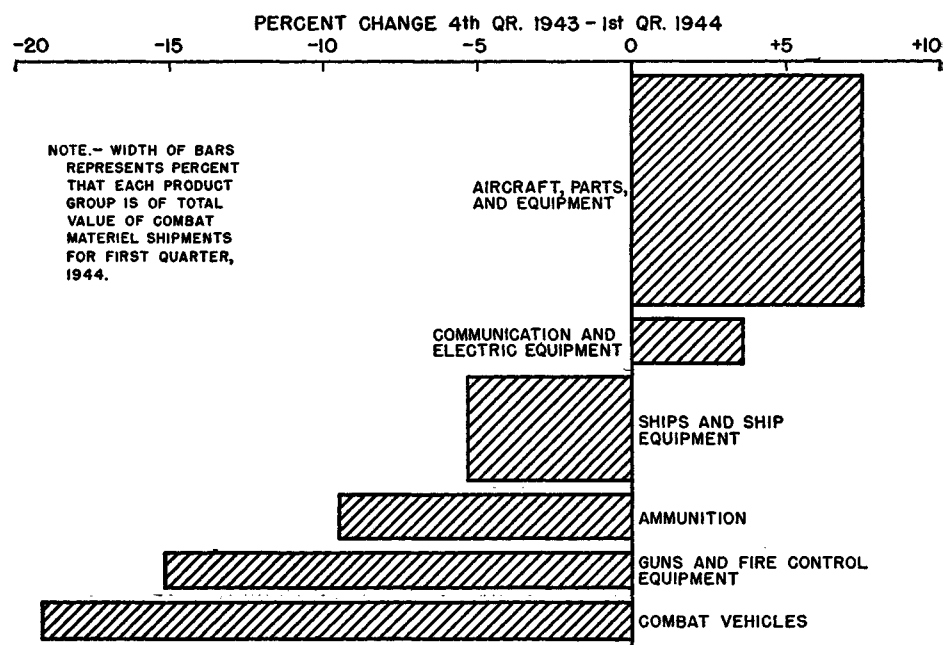
Chart 1.—Percentage Change in Value of Combat Matériel Shipments From Metal-Producing Manufacturing Plants
