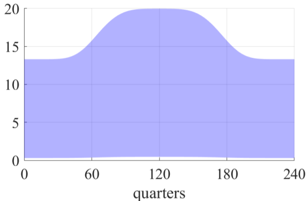
FIGURE: The mass of endowment profiles: e_{s,i} \sim e_s \cdot \mathcal{U} [\bar{\zeta}^{-1}, \bar{\zeta}] , e_s = 2 + \exp \left[ - \left( \frac{s-120}{60} \right)^4 \right] , \bar{\zeta} = 6.5 .
