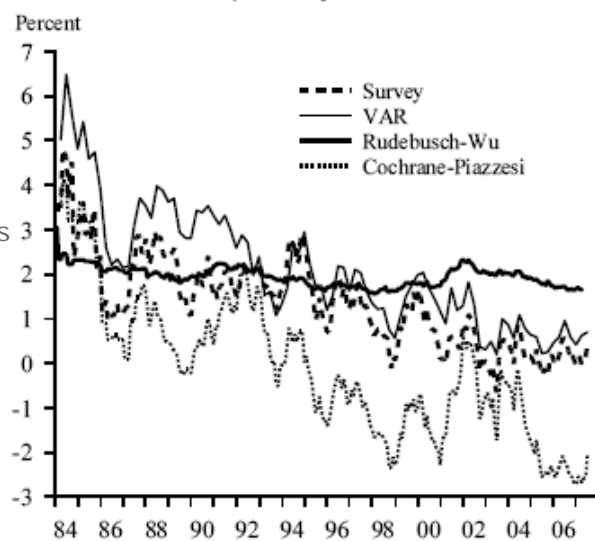
Figure 1 Four measures of the 10-year term premium
