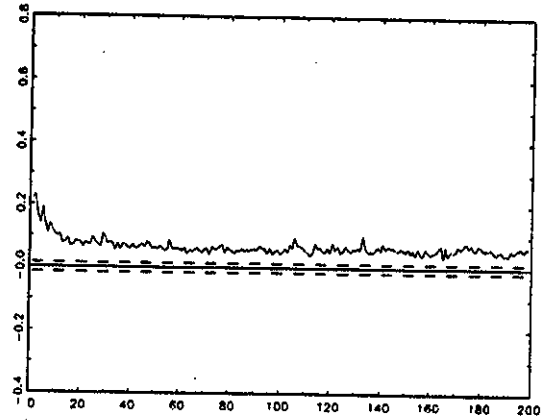
Autocorrelation Function-S&P \epsilon^2 - Jan 28 to May 90
