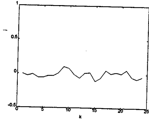
Sample Autocorrelation Function
