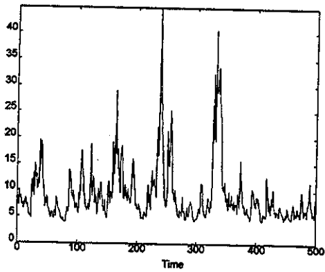
Conditional Variance
