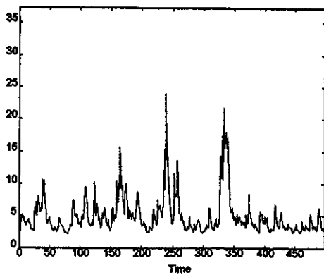
Conditional Covariance
