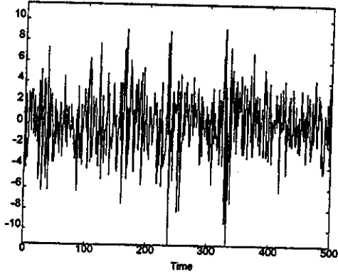
GARCH(1,1) Realization
