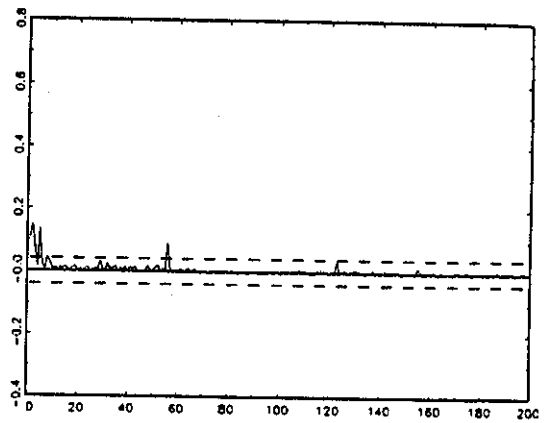
Autocorrelation Function-S&P \epsilon^2 - Jan 81 to May 90
