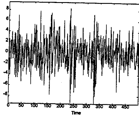
Factor-GARCH Series 2
