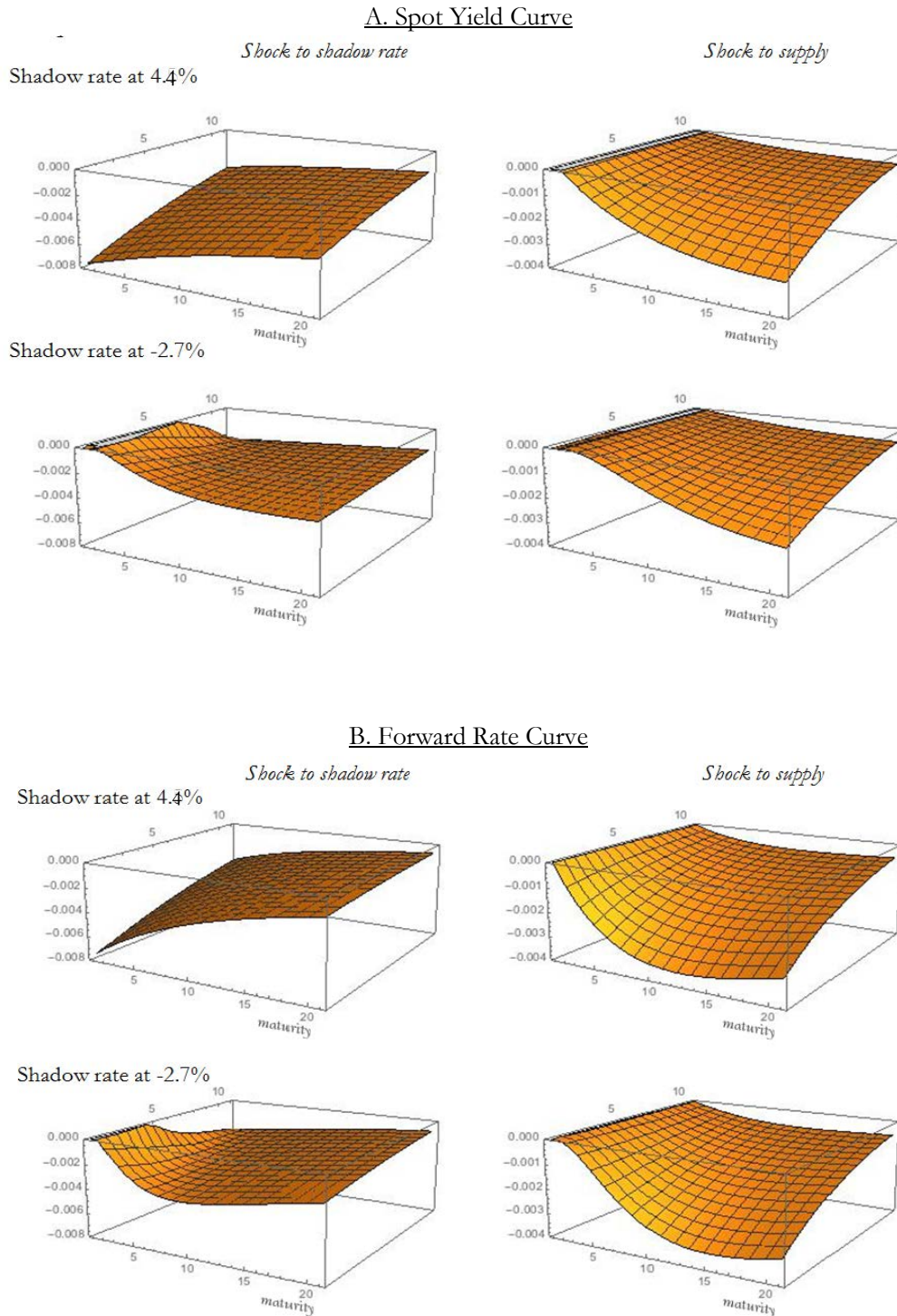
Figure 6. Impulse-Response Functions
