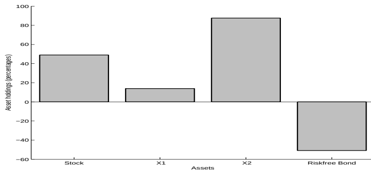
Figure 2: The components of human capital. The histogram depicts the investments in the various securities (risky asset S , pseudo-securities X_j , j = 1, 2 , and risk-free money market B ) that replicate the long position in human capital (that is, the present value of future labor income flows).
