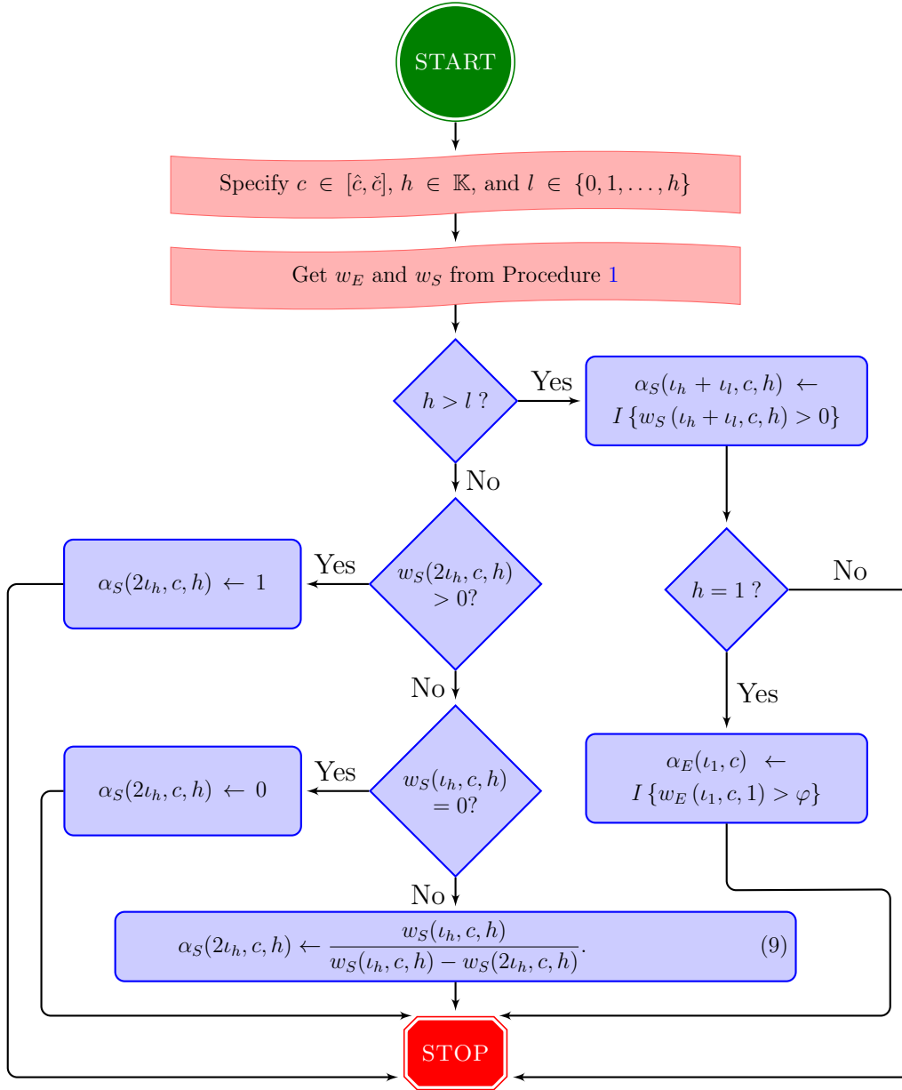
Procedure 2: Calculation of Candidate Survival Rule for the Heterogeneous Duopoly Model
