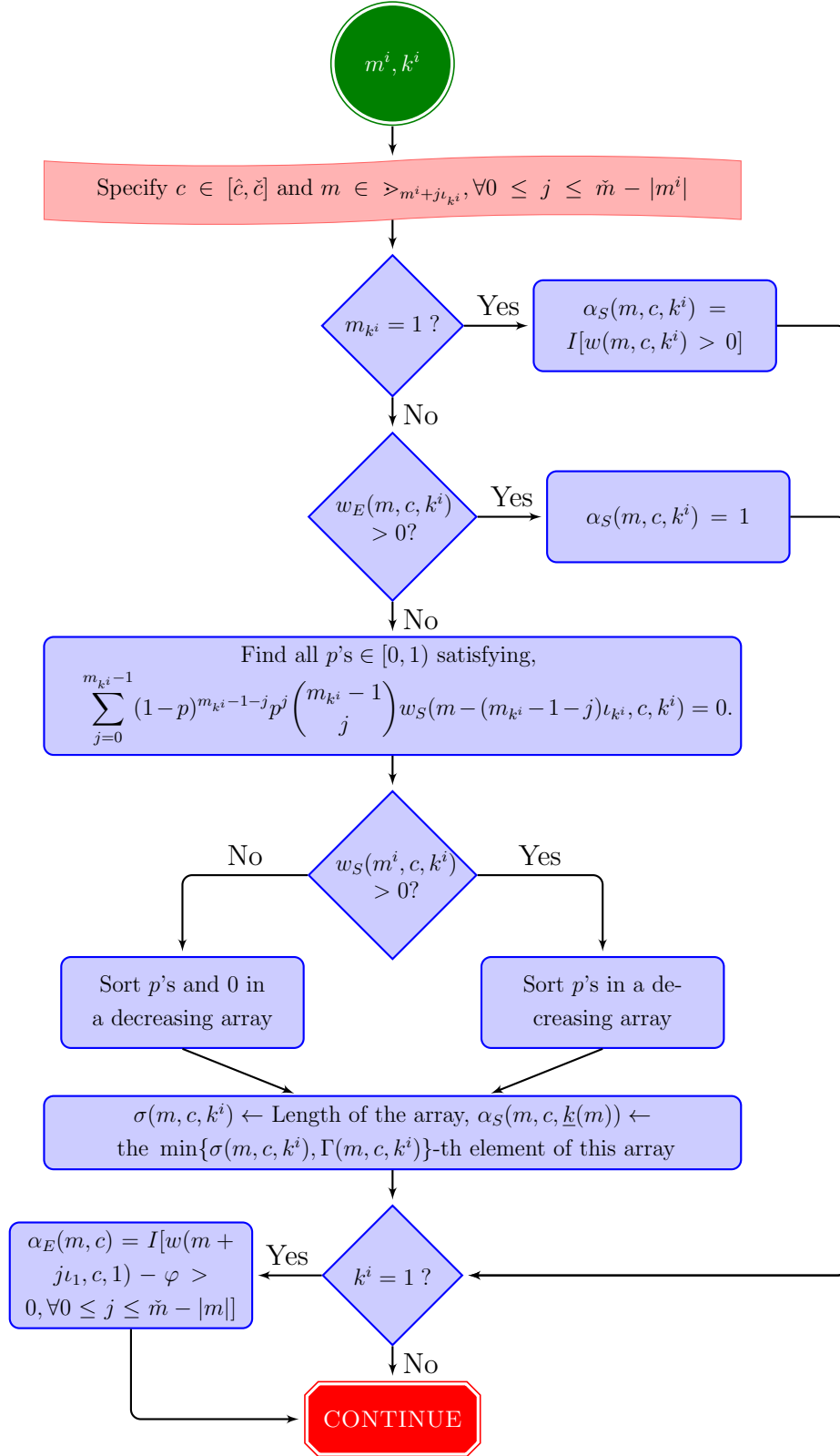
Procedure 3: Calculation of Candidate Entry/Survival Rule for the General Model, Non-Monotone Payoffs
