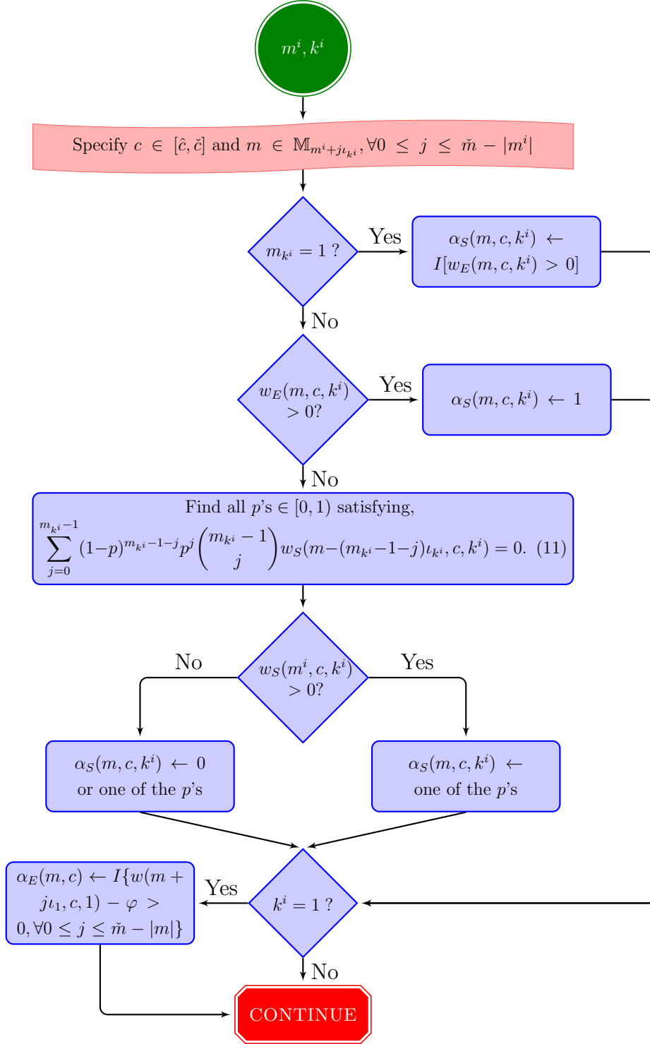
Procedure 3: Calculation of Candidate Entry/Survival Rule for the General Model
