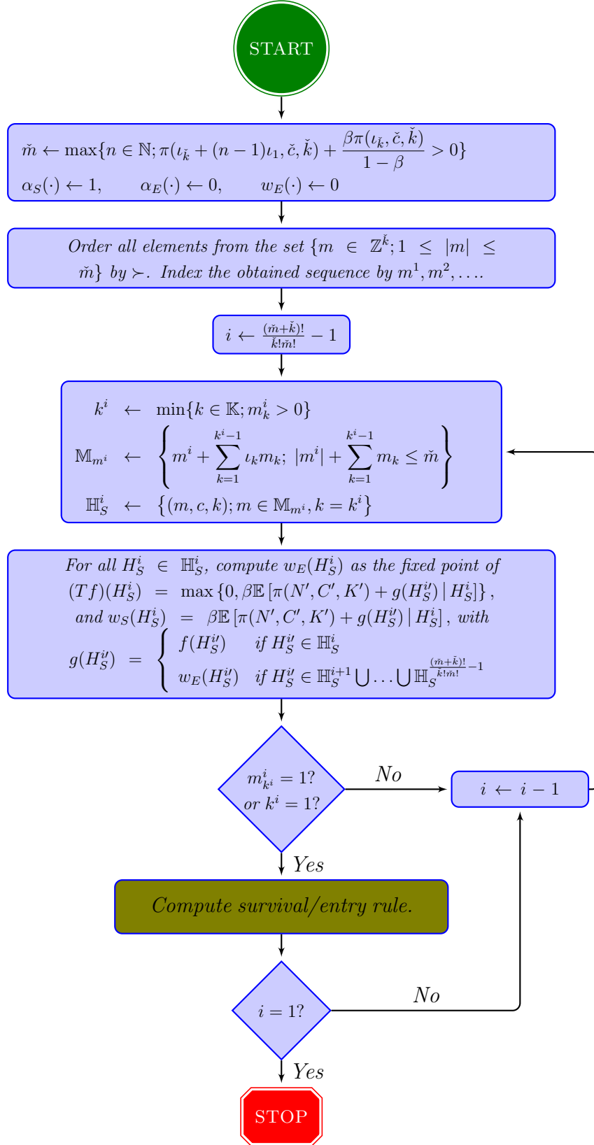
Algorithm 2 (Calculation of a Candidate Equilibrium for the General Model).
