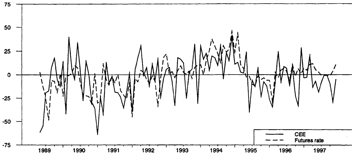
Figure 3: Forecast one-month change in the Fed funds rate
