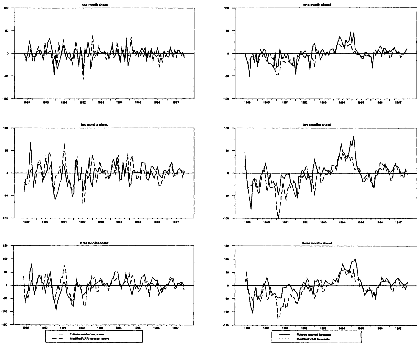
Figure 4: Forecasts and errors from modified VAR equation
