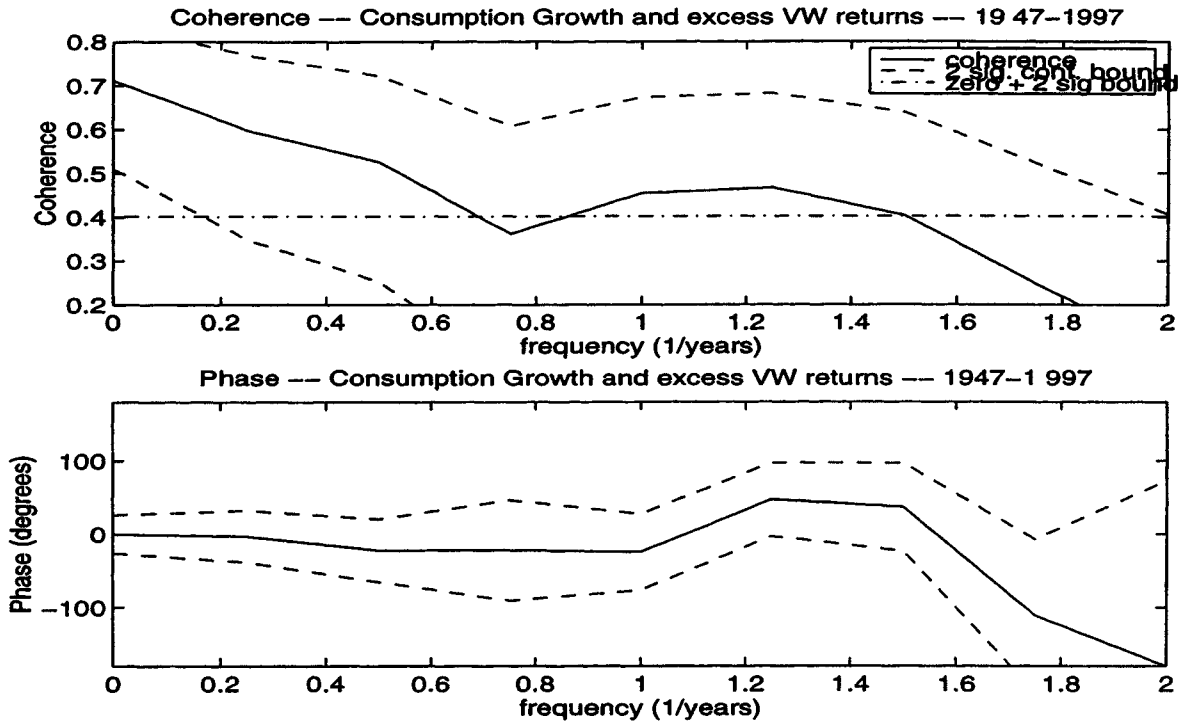
Figure 2: Coherence and Phase plots for Consumption Growth and Lagged excess VW index Returns
