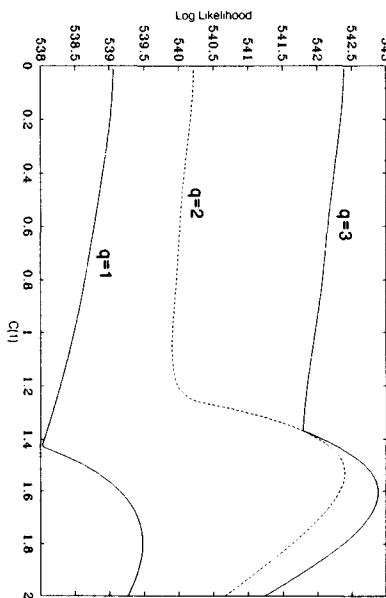
Figure 1c ARMA(2,q)
