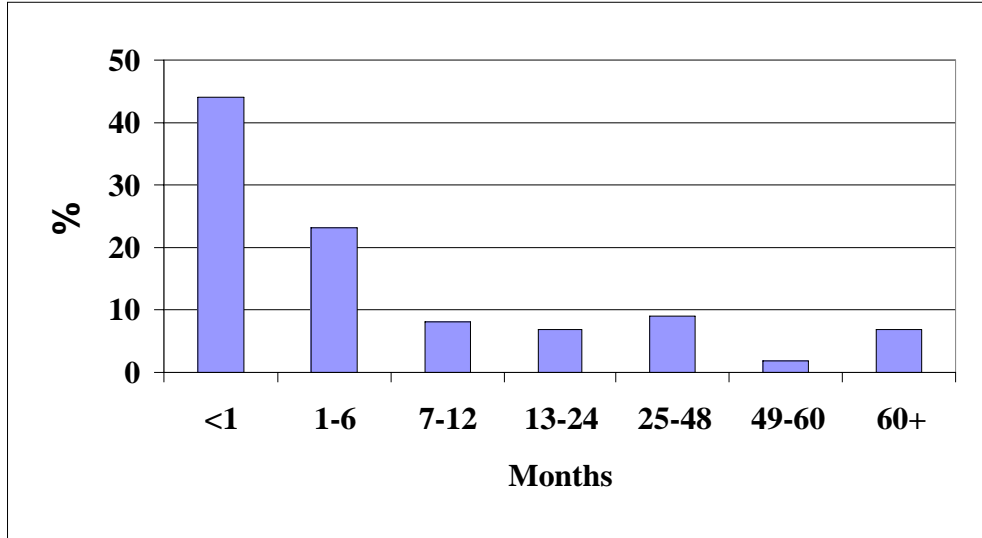
Figure 3 Lag Time In ID Theft Discovery
