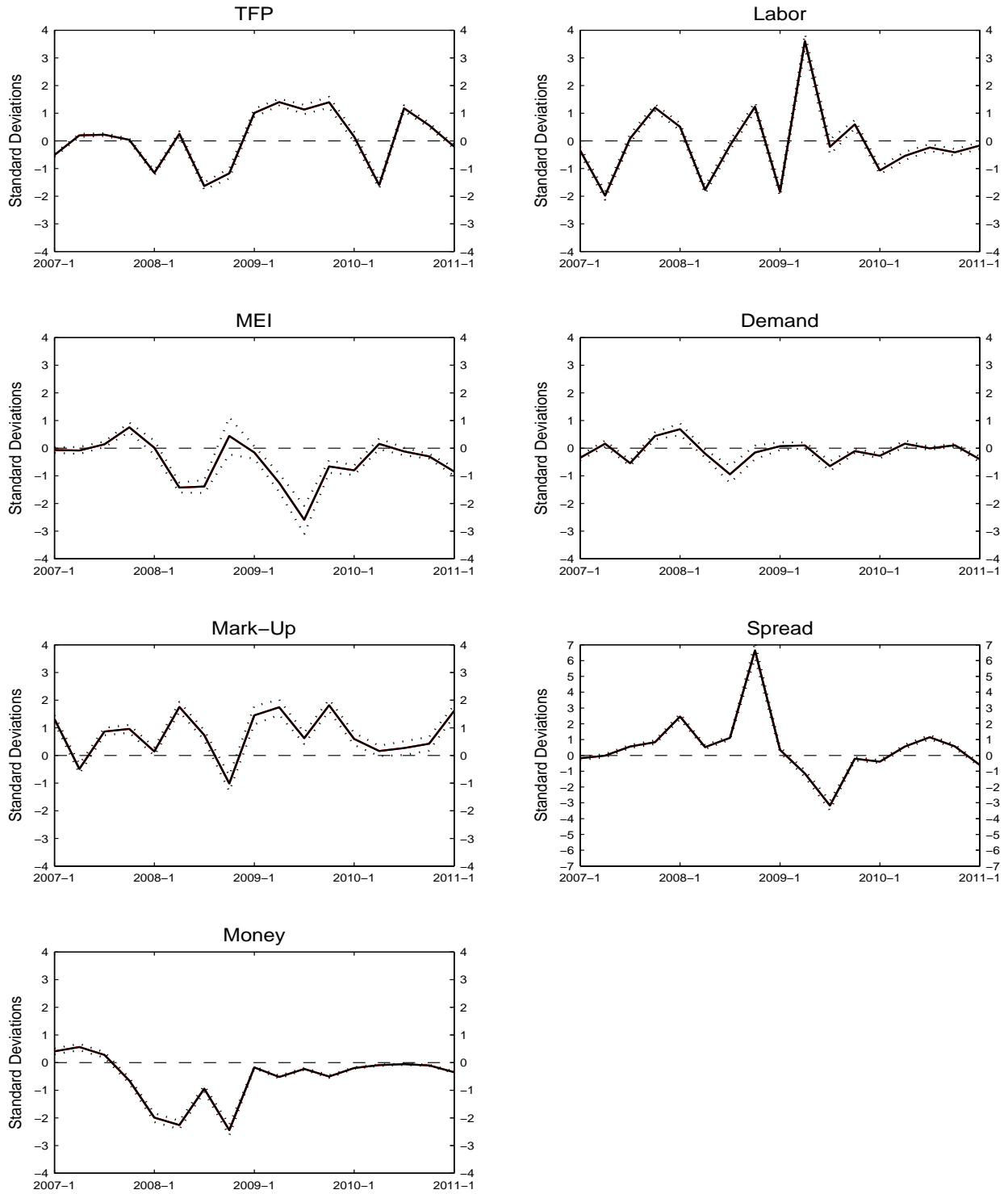
Figure 4: Shock Histories
