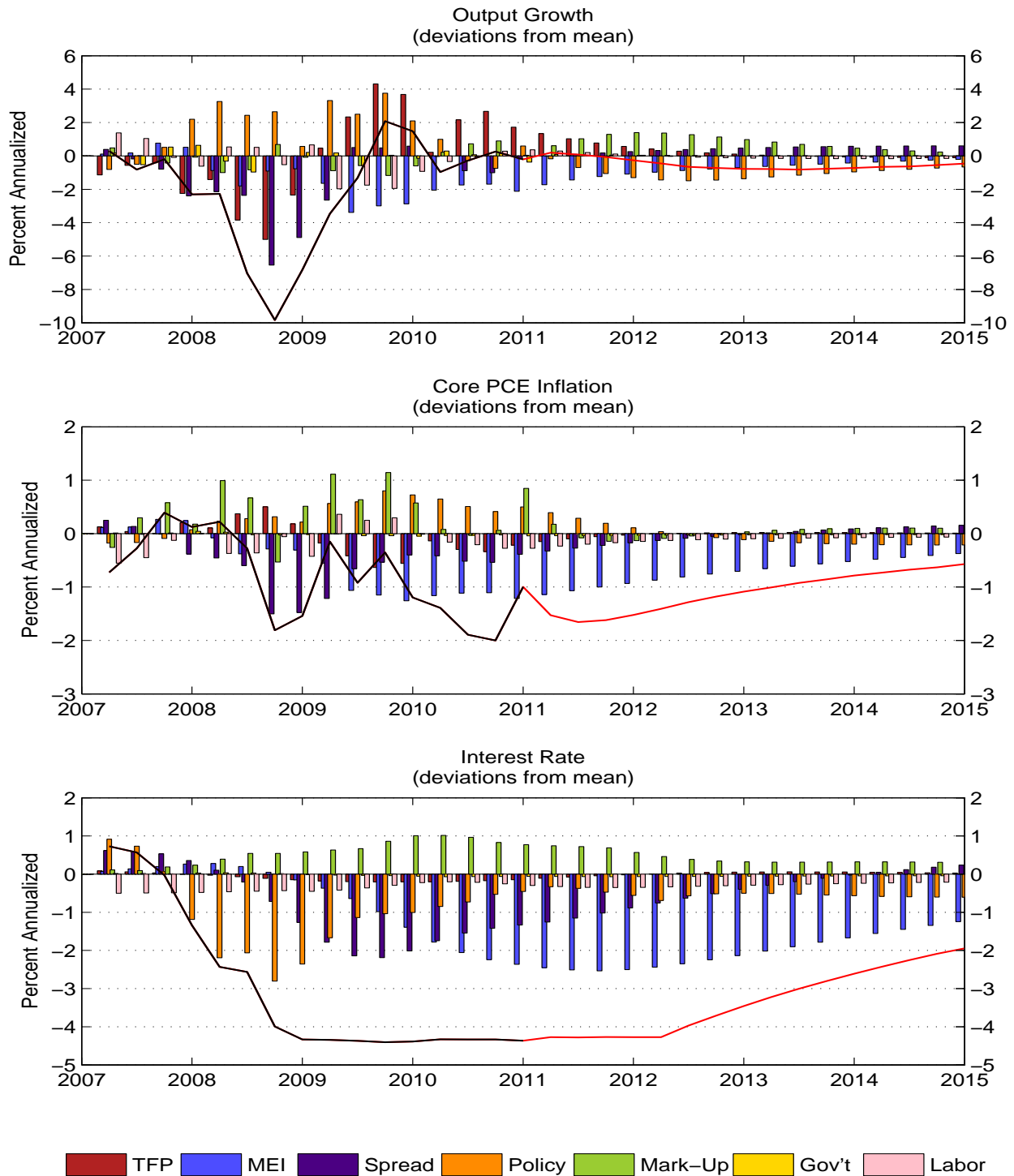
Figure 2: Shock Decomposition
