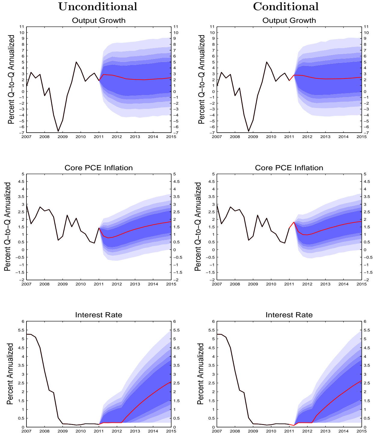
Figure 3: Forecasts
