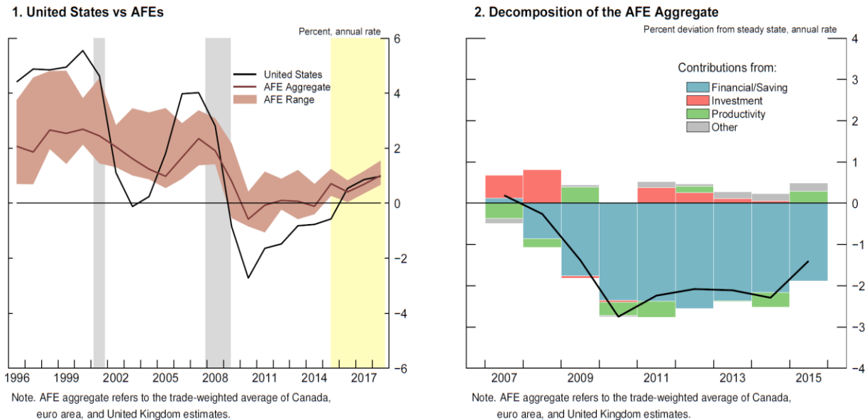
Figure 4: The real natural rate of interest in the AFEs
