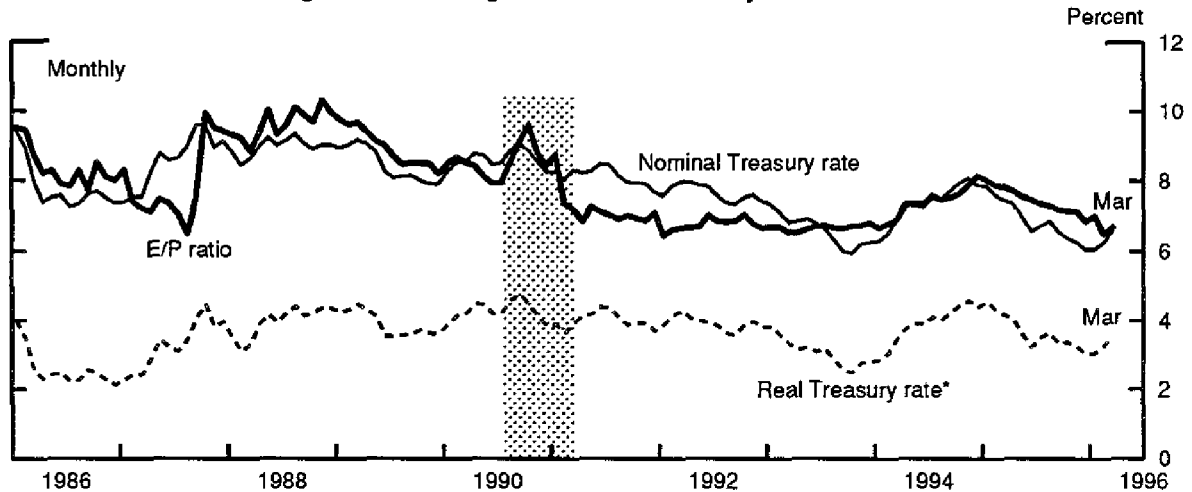
12-Month Forward Earnings-Price Ratio Against 30-Year Treasury Rate
