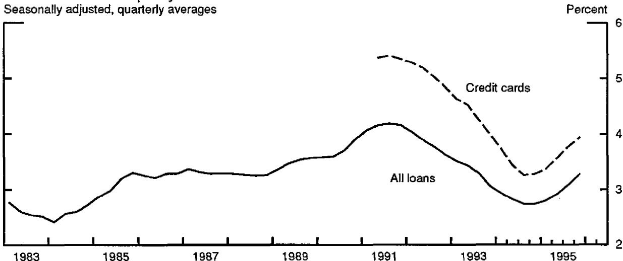
Consumer Loan Delinquency Rates at Banks Seasonally adjusted, quarterly averages
