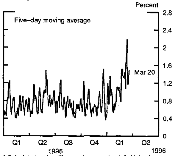
Volatility of the S&P 500*
