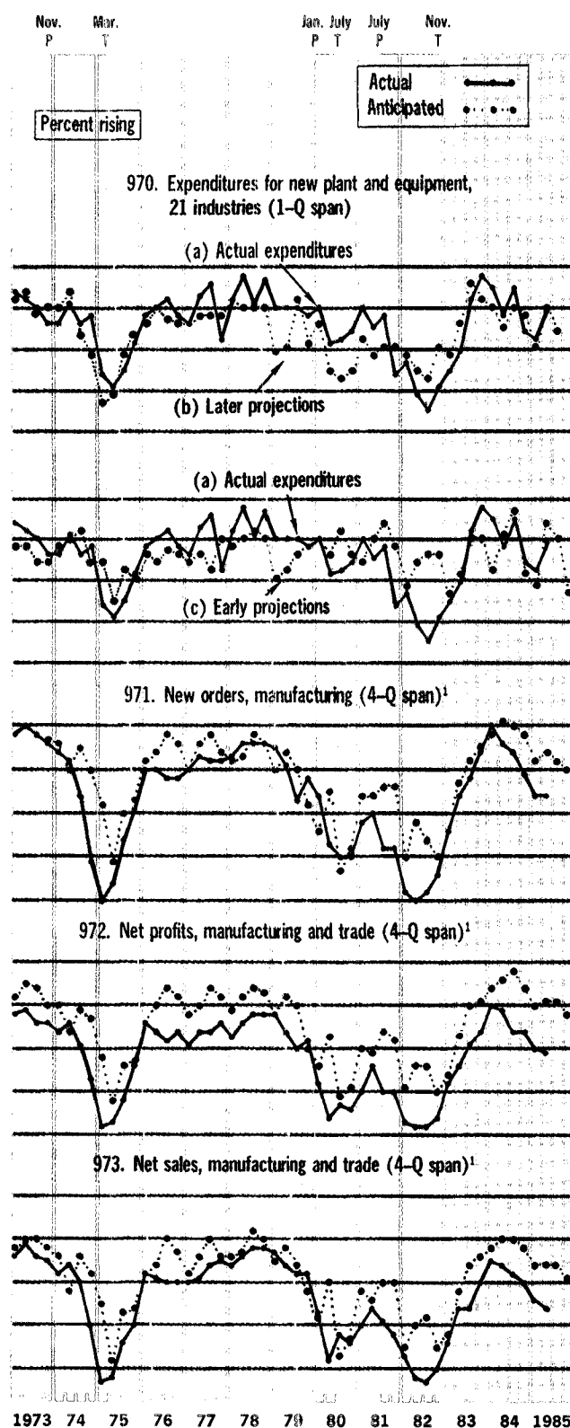
Chart C1. Diffusion Indexes—Continued
